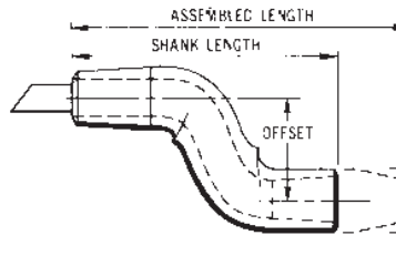
SHANKS 5 RW TAPER
