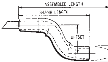
SHANKS 4 RW TAPER
