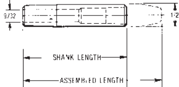
SHANKS 5 RW TAPER
