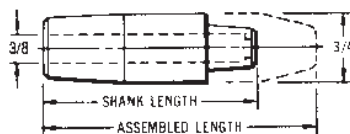
SHANKS 6 RW TAPER
