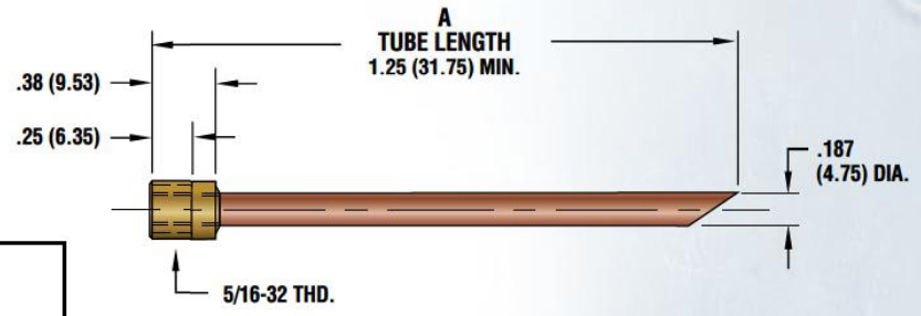
FIGURE 8-9 (Material - Copper & Brass)
