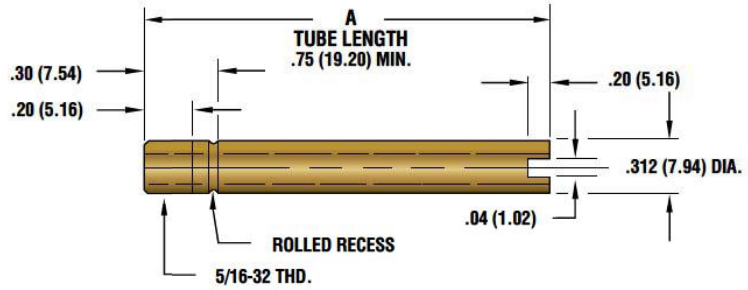
FIGURE 8-1 (Material - 1/4 ID BRASS TUBE)
